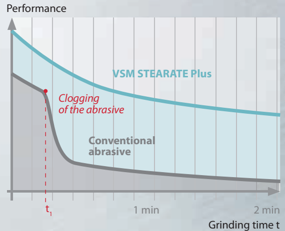
Grinding bars (Ø 30 mm) made of aluminium alloy (AlSi12Cu) using fibre discs with grit size 24.
