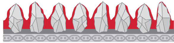
Standard coating, closed-coated
